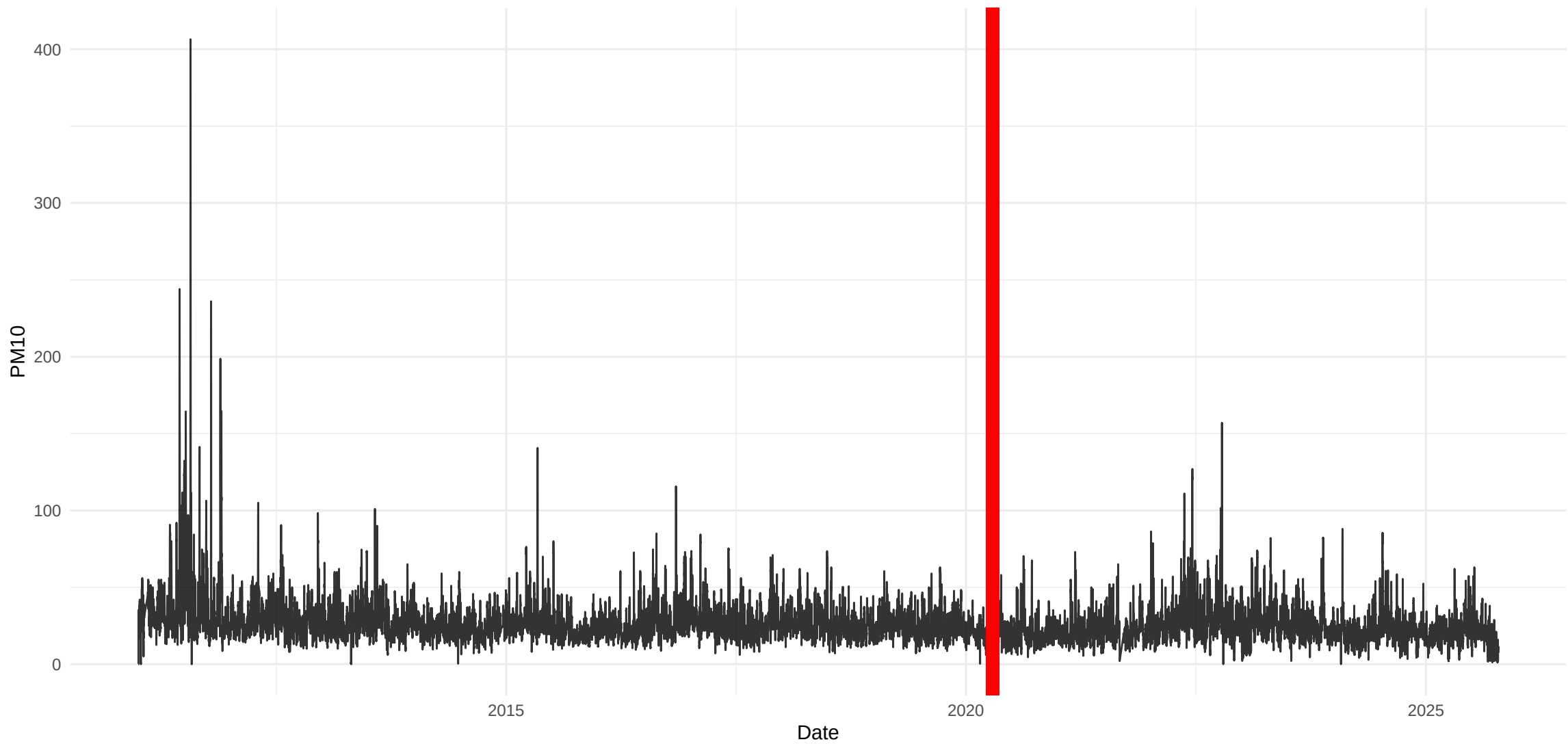
Time Series of PM10
