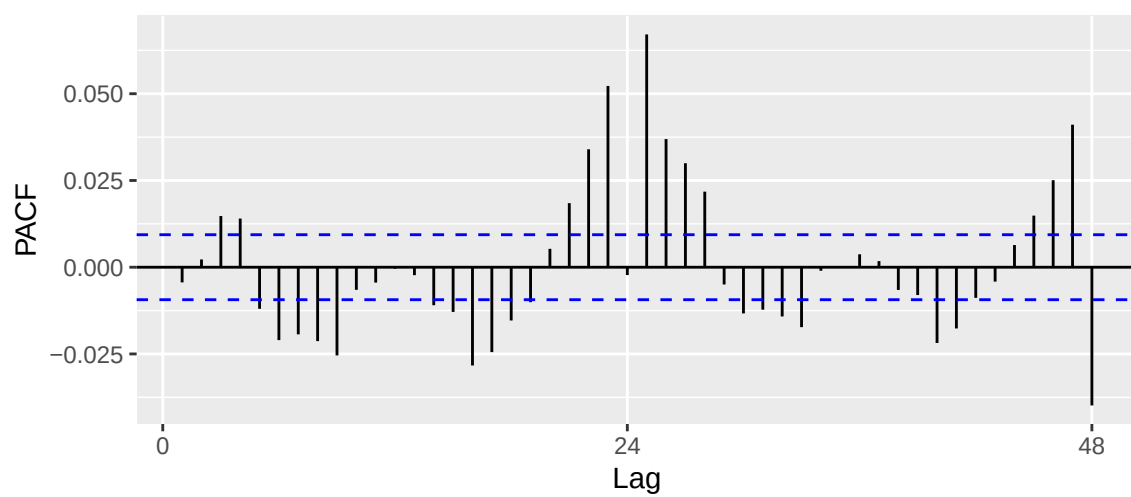
PACF of Residuals for CO
