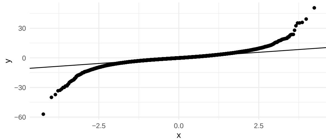
Q-Q Plot of Residuals for NO2
