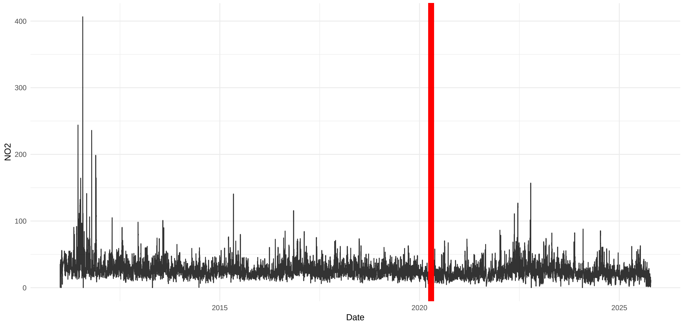
Time Series of NO2
