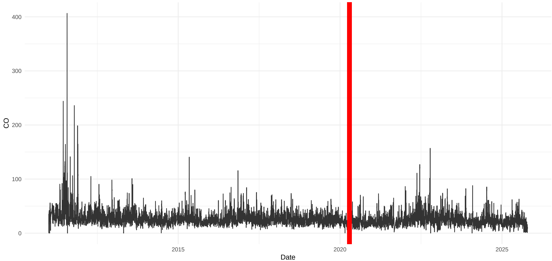
Time Series of CO
