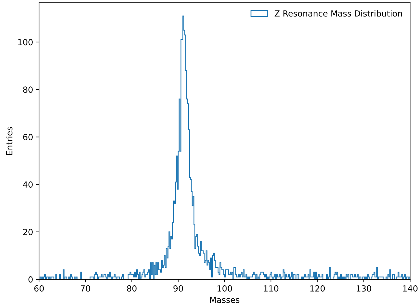
Z Resonance Mass Distribution
