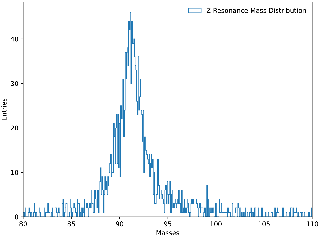
Z Resonance Mass Distribution
