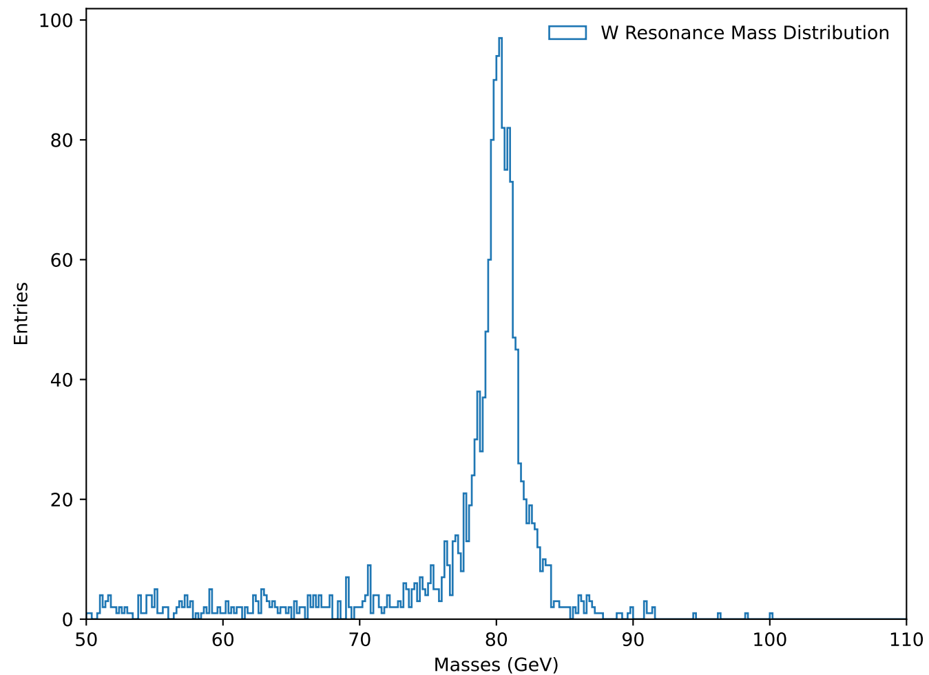
W Resonance Mass Distribution
