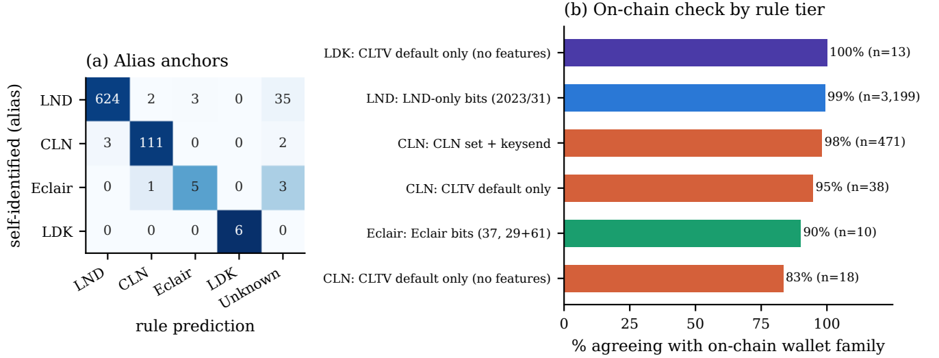
Fig. 1. Validation of client inference. (a) Nodes whose alias names their implementation vs. the rule label. (b) Share of nodes in each rule tier whose channel-funding wallet agrees with the label (tiers with n \geq 10 ).
