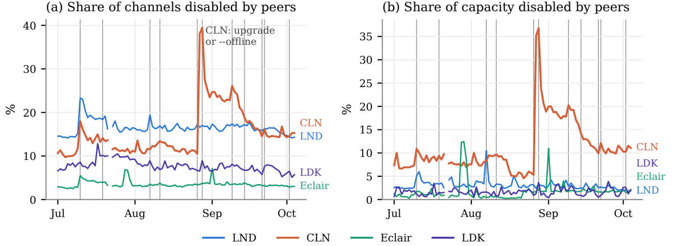
Fig. 3. Share of channel directions toward each client’s nodes that peers mark disabled, daily, July–October 2026; by channel count (a) and by capacity (b). Vertical lines: events of §VI.
