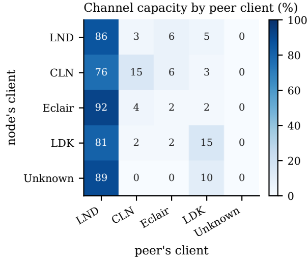
Fig. 8. Share of each client's channel capacity (rows) by the client of the peer (columns), routable core of 25 August 2026.
