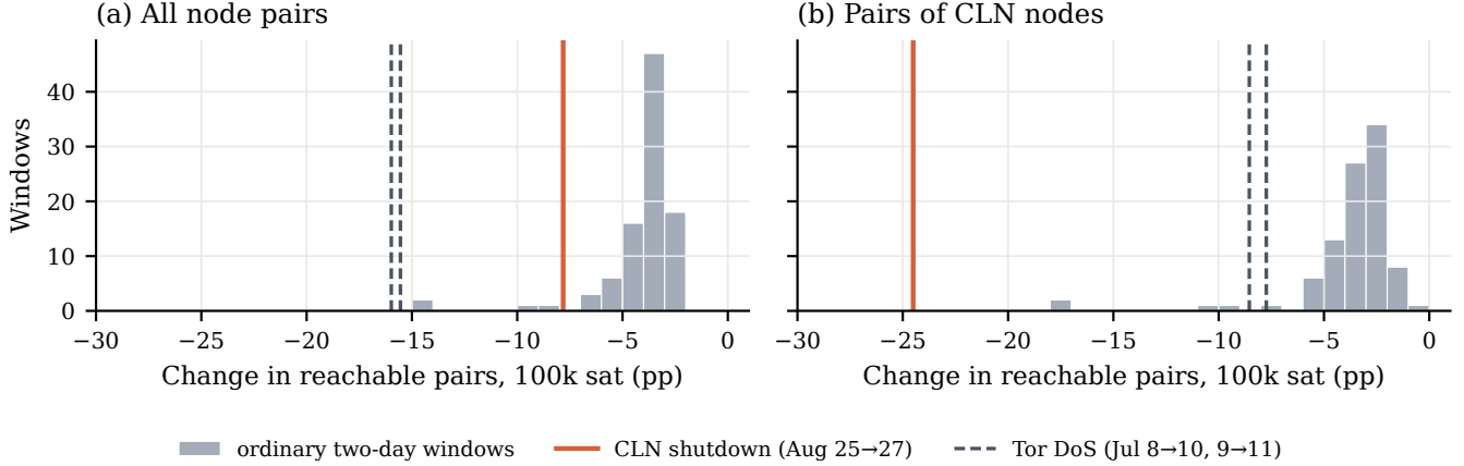
Fig. 6. Change in the share of pre-failure node pairs that can still route 100k sat, from each gossip snapshot to the one two days later (nodes that lost every usable channel count as failed), May–August 2026. Grey: windows without a known incident; solid line: 25→27 August (CLN shutdown); dashed: 8→10 and 9→11 July (Tor denial-of-service wave). (a) All node pairs; (b) pairs of CLN nodes.
