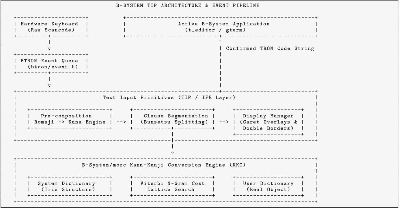
Figure 1: System event routing and pipeline architecture of the B-System Text Input Primitives (TIP).
