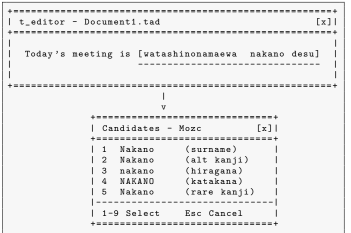
Figure 2: Visual layout of inline composition and candidate selection window in B-System.
