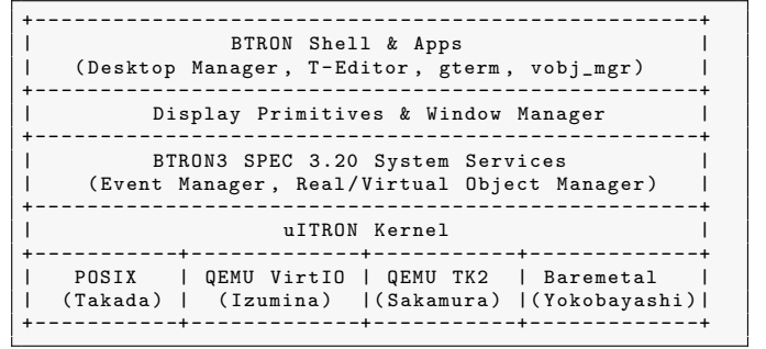
Figure 2: Layered architecture and target execution matrix.
