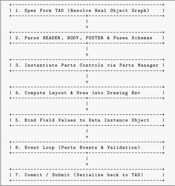
Figure 3: Seven-phase runtime execution lifecycle of a form.
