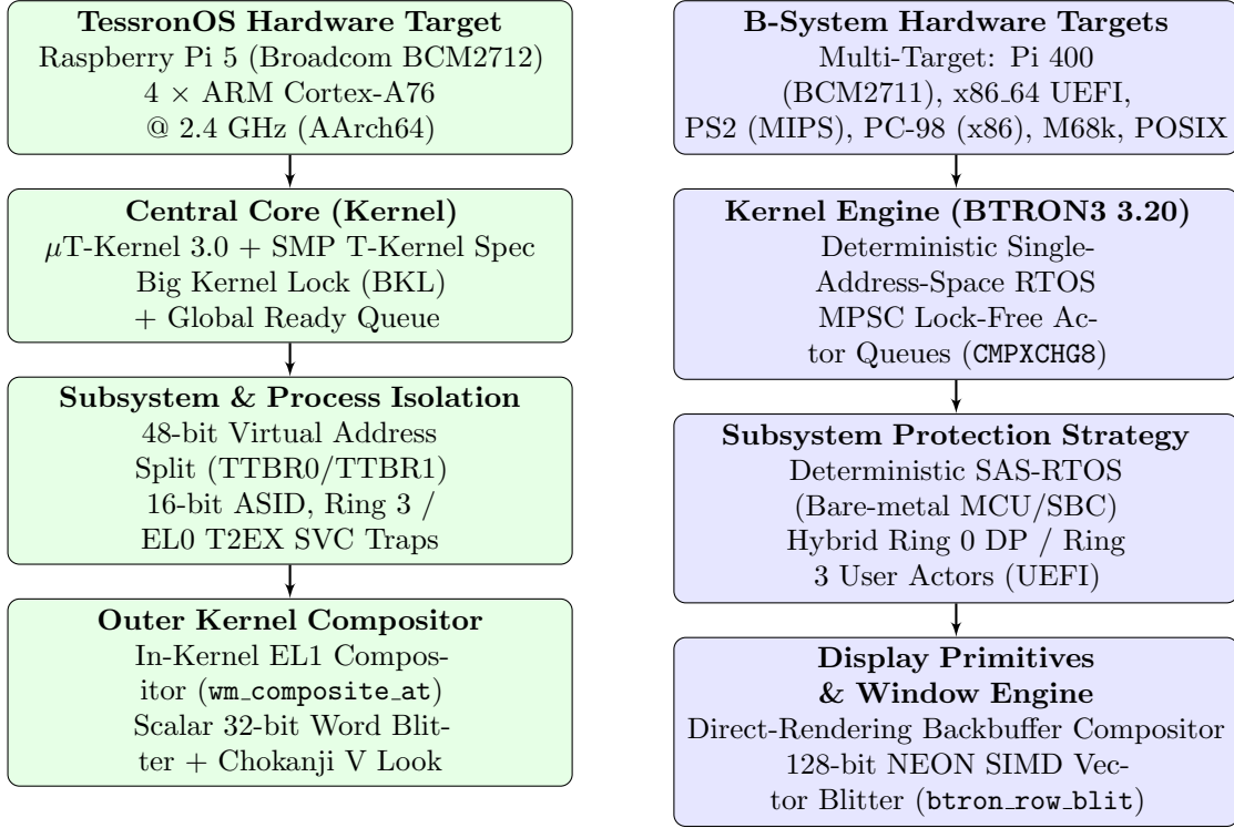
Figure 1: Architectural topologies of satromi’s TessronOS (evolutionary \mu T-Kernel 3.0 / SMP T-Kernel / T2EX lineage) versus 5HT’s B-System (cleanroom BTRON3 3.20 multi-target unikernel / RTOS engine).
