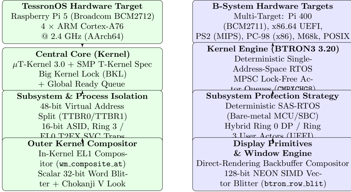
Figure 1: Architectural topologies of satromi’s TessronOS (evolutionary \mu T-Kernel 3.0 / SMP T-Kernel / T2EX lineage) versus 5HT’s B-System (cleanroom BTRON3 3.20 multi-target unikernel / RTOS engine).
