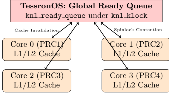
Figure 2: Cache-line bouncing and lock contention in TessronOS's single global ready queue architecture.
