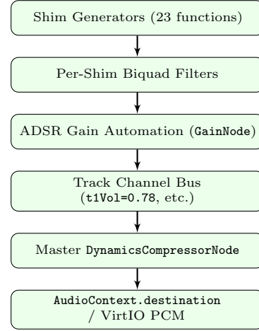
Figure 6: BTRON master audio signal flow graph.
