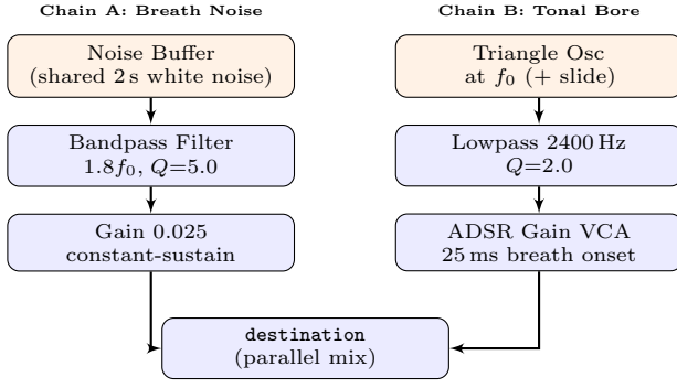
Figure 5: shimSaxFlute : dual parallel source chains. Chain A (breath turbulence) is a sustained bandpass-filtered noise at 1.8f_0 , Q=5 running for the full note duration. Chain B (tonal bore) is a triangle oscillator through a 2400 Hz lowpass, giving the hollow flute timbre. Both chains sum at AudioContext.destination with a -16 dB noise-to-tone ratio.
