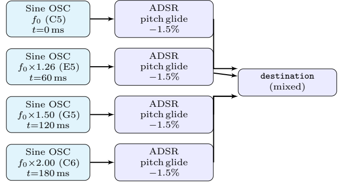
Figure 2: shimFloat : four-voice polyphonic chord fan. Each sine OSC fires at a staggered offset of 60 ms, producing the characteristic wrist-roll of the Imada Fender Rhodes chord voicing. All four ADSR chains share the same -1.5\% pitch glide (40 ms settle) and converge at AudioContext.destination .
