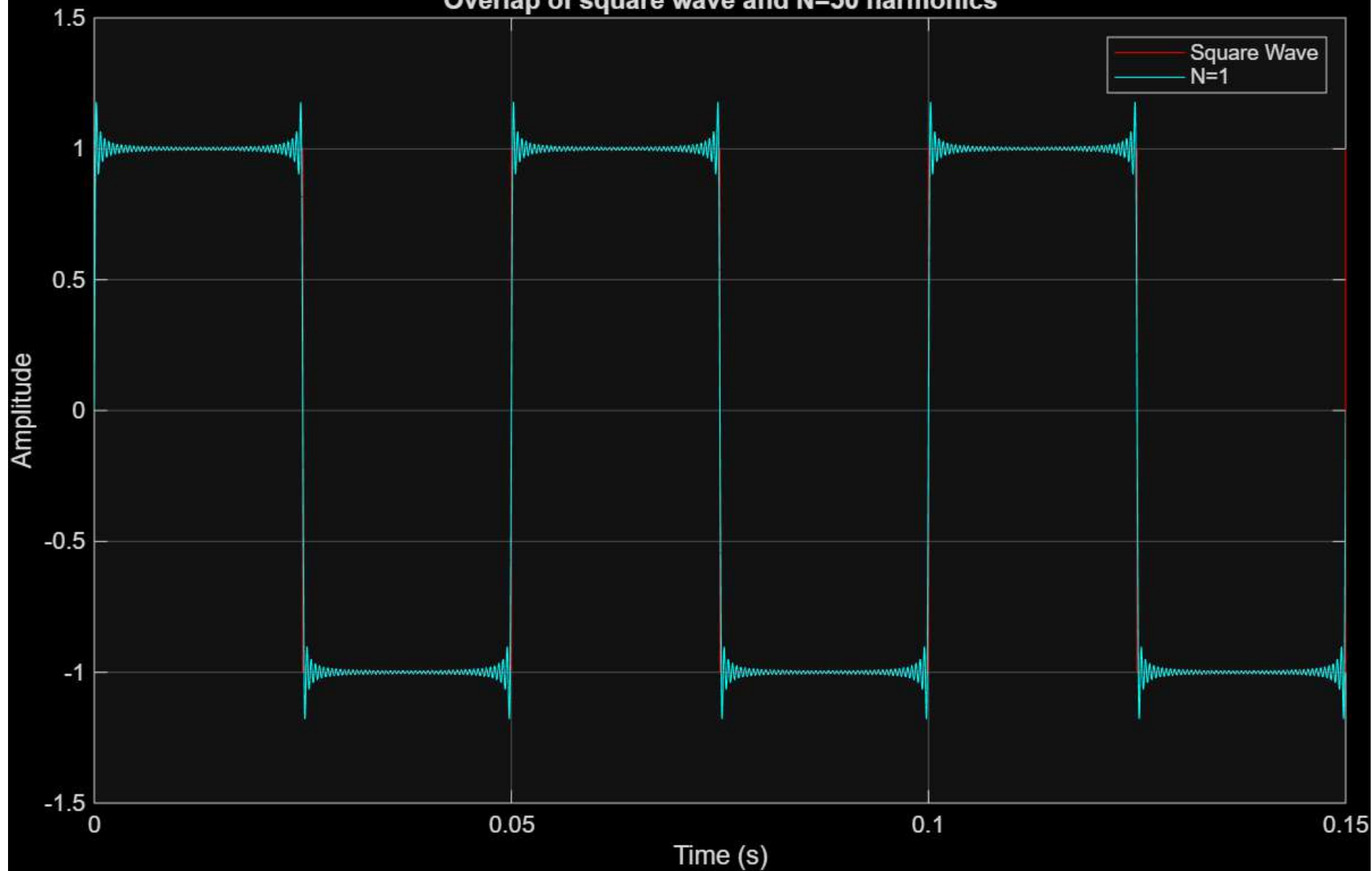
Overlap of square wave and N=50 harmonics
