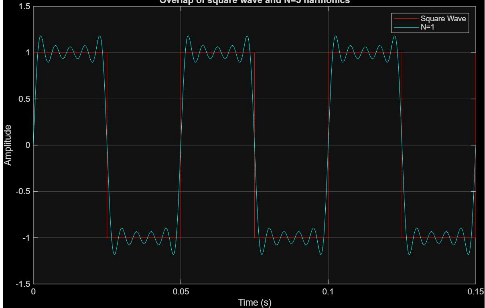
Overlap of square wave and N=5 harmonics
