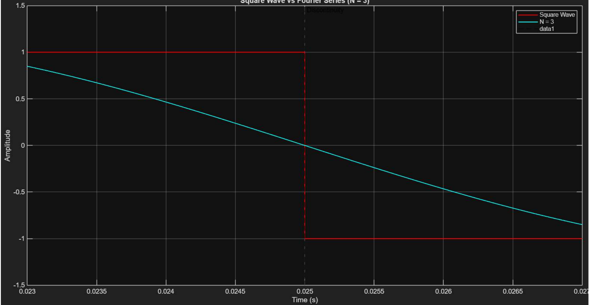
Square Wave vs Fourier Series (N = 3)
