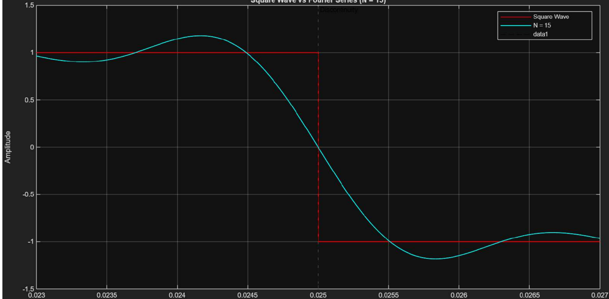
Square Wave vs Fourier Series (N = 15)
