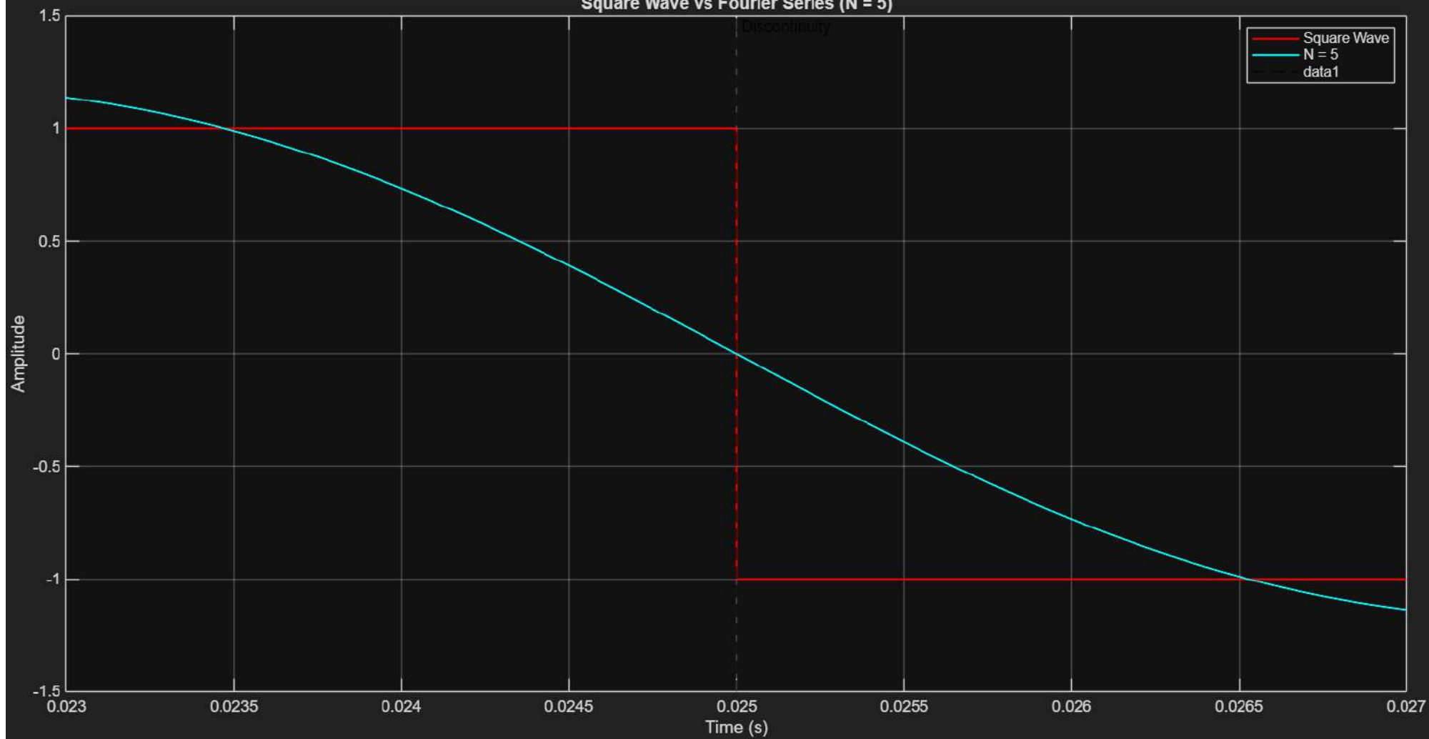
Square Wave vs Fourier Series (N = 5)
