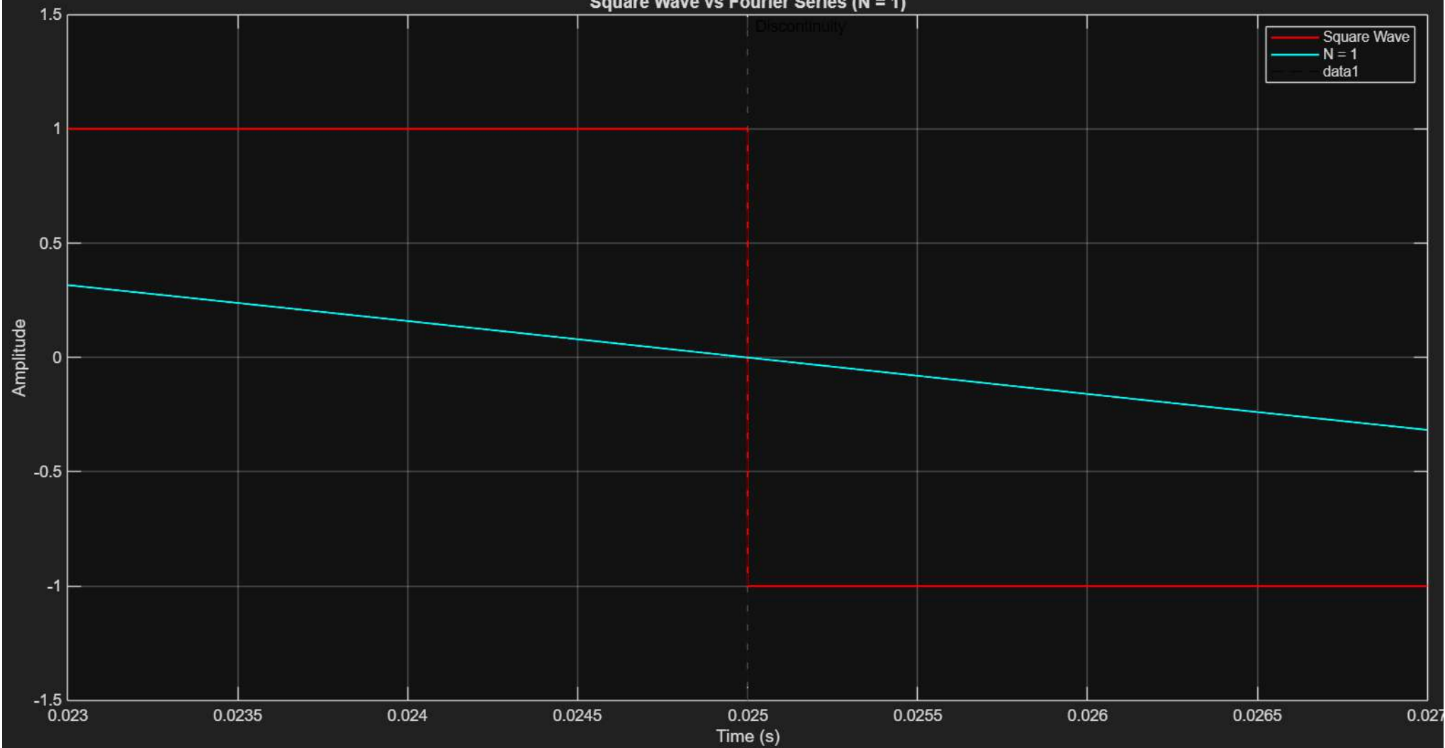
Square Wave vs Fourier Series (N = 1)
