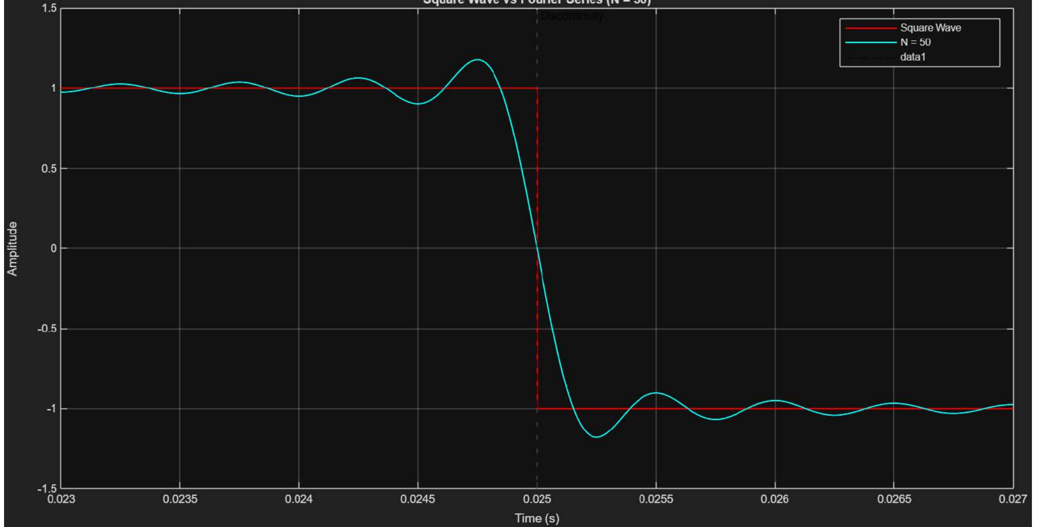
Square Wave vs Fourier Series (N = 50)
