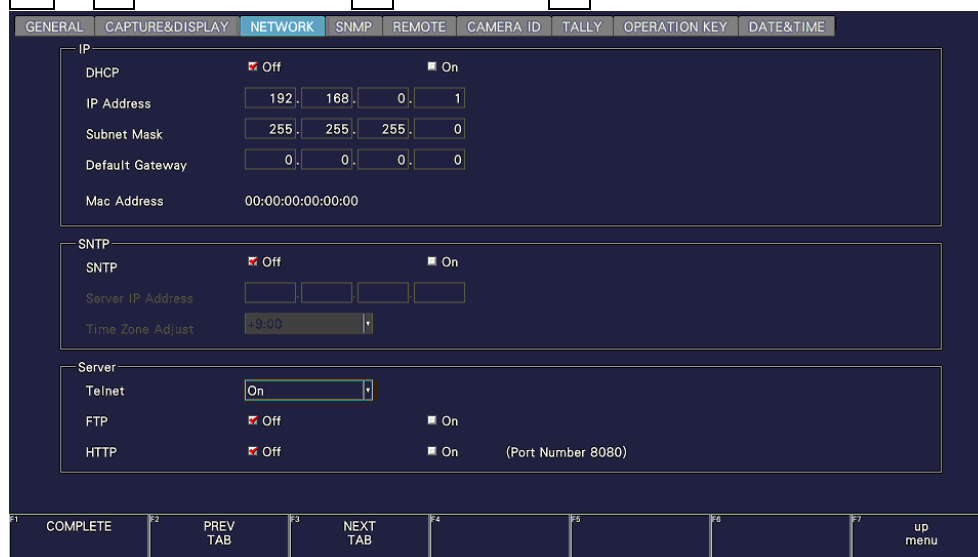
Figure 19-2 NETWORK tab
