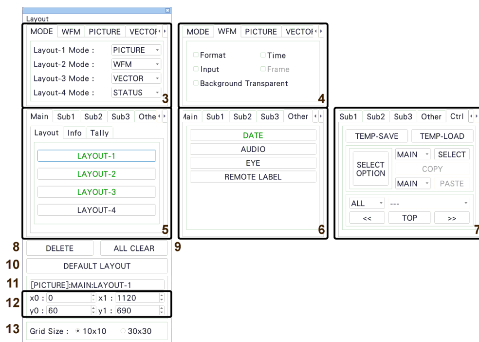
Figure 6-59 Enhanced layout window
