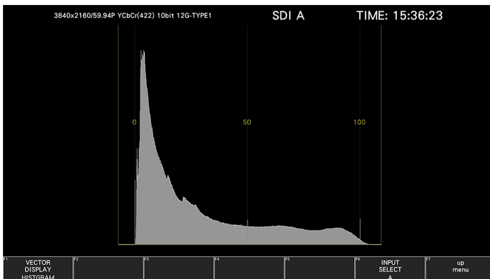
Figure 11-26 Histogram Display
