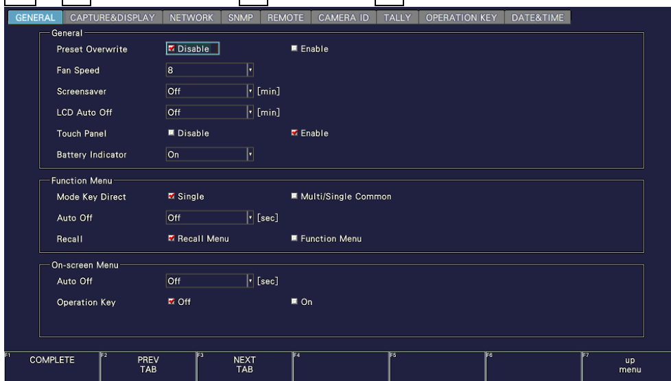
Figure 7-11 GENERAL tab
