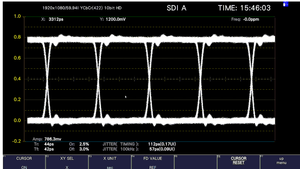
Figure 17-21 Cursor display
