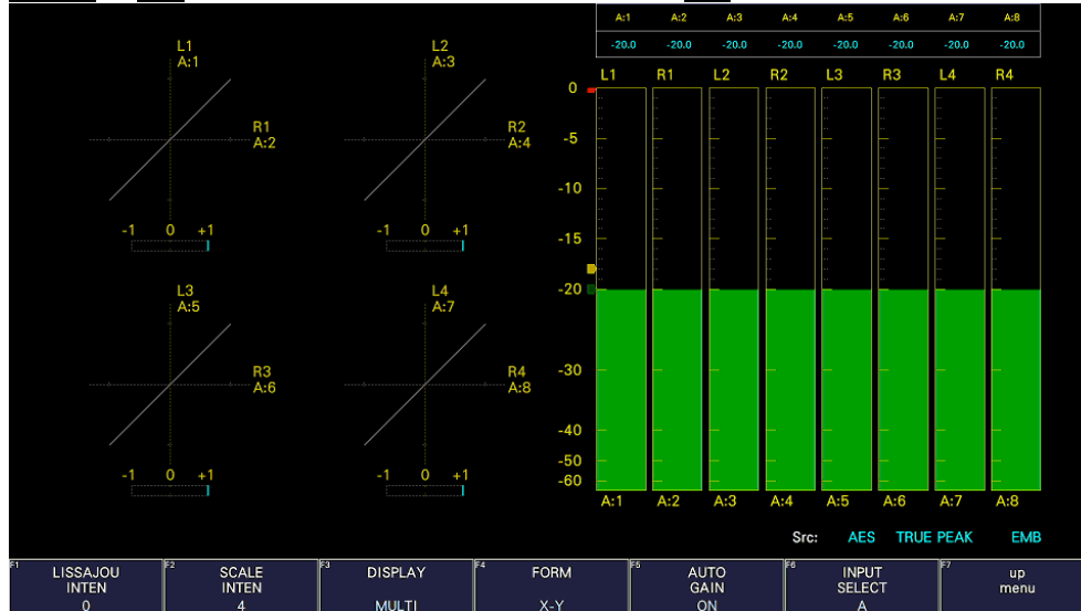
Figure 15-9 Lissajous display
