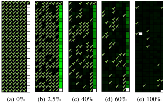
FIGURE 10: Time-series visualization of SSD block states during MSR prxy workload execution with 5% OPS, showing progression from initial state (0%) to completion (100%). Demonstrates how invalid pages gradually spread from OPS-reserved region to entire SSD, causing WAF increase. (The darkest green block: the most valid pages, the brightest green: the most invalid pages, cross-signed blocks: fully invalid, and tick-signed: fully valid)
