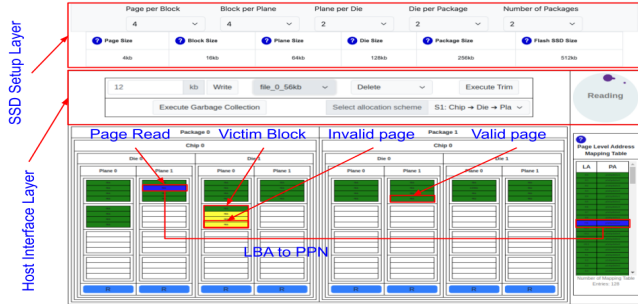
FIGURE 2: Web interface of the basic SSD simulator showing user controls for I/O operations, allocation scheme selection, and real-time visualization of write count (WC), read count (RC), erase count (EC), and WAF metrics
