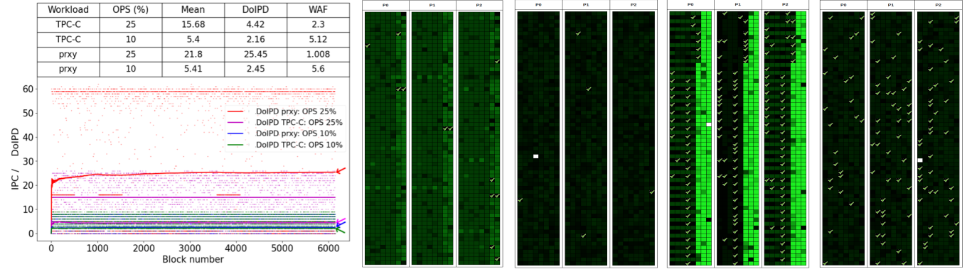
FIGURE 9: (a) Scatter plot of invalid page counts per block with cumulative DoIPD lines for TPC-C and prxy workloads at different OPS levels; (b-e) corresponding SSD block state visualizations showing the impact of OPS on data clustering. (The darkest green block: the most valid pages, the brightest green: the most invalid pages, cross-signed blocks: fully invalid, and tick-signed: fully valid)
