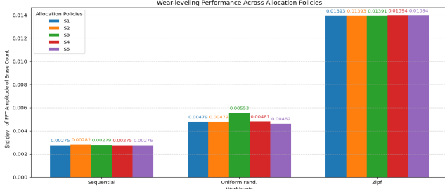
FIGURE 7: Bar chart comparing standard deviation of Fourier Transform amplitudes ( \sigma_A ) across five allocation policies (S1–S5) for sequential, uniform random, and Zipf workloads. Lower \sigma_A values indicate more uniform erase count distribution and better wear-leveling performance.
