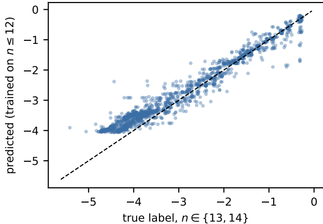
HGB: R^2 = 0.91
