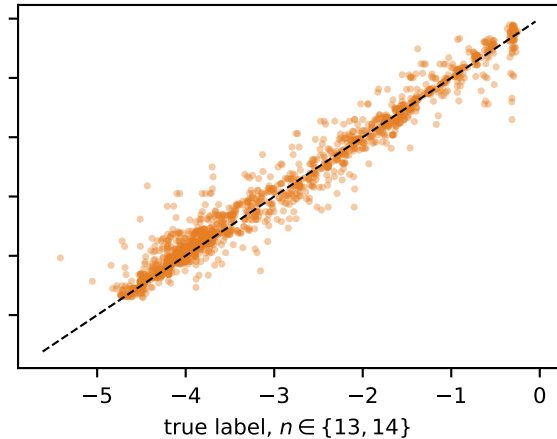
MLP: R^2 = 0.97
