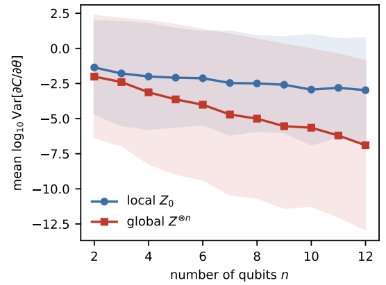
FIGURE 3. Mean \log_{10} \text{Var}[\partial C / \partial \theta] vs. qubit count for local and global cost observables (shaded: \pm 1 standard deviation). Global costs show the exponential decay characteristic of barren plateaus.
