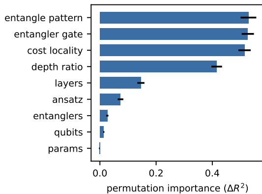
FIGURE 4. Permutation feature importance for the trainability regressor. Cost locality and entanglement structure dominate.
