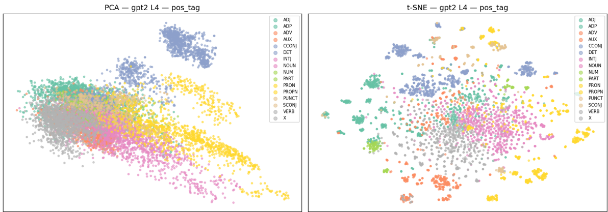
(b) GPT-2 L4: PCA shows an elongated manifold with a function-word-to-content-word gradient; t-SNE clusters are comparably clean, with DET, ADP, and PRON forming particularly tight groups.
