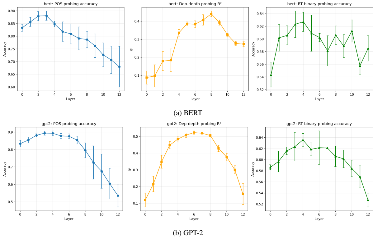
Figure 1: Layer-wise probing: POS accuracy (blue), dep-depth R^2 (orange), RT binary accuracy (green), \pm 1 SD across 3-fold CV. POS peaks early (L3–4), dep-depth peaks mid (BERT L8, GPT-2 L6), RT peaks at L4. GPT-2 shows steeper late-layer collapse for all three probes.
