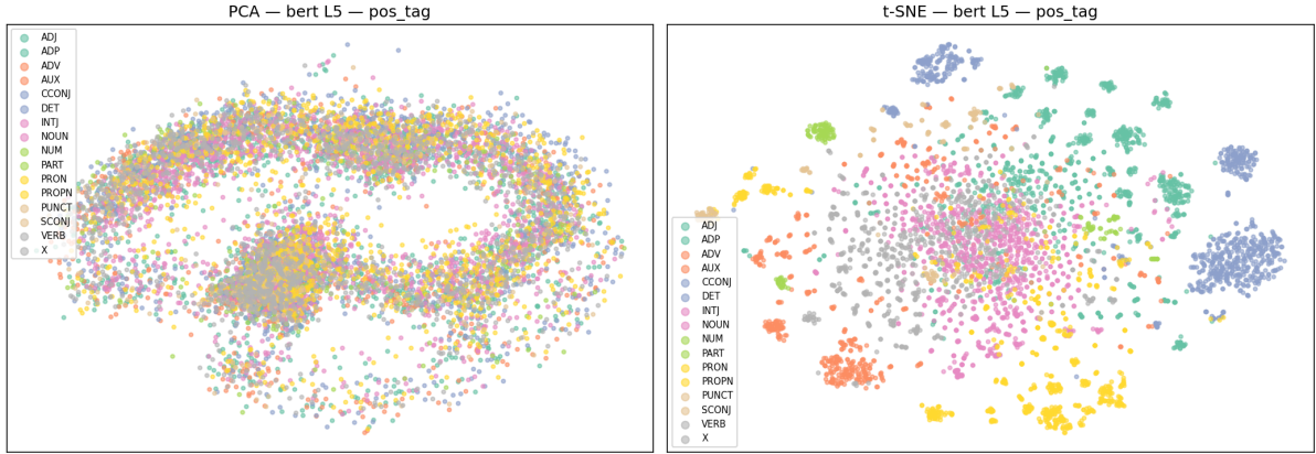
(a) BERT L5: PCA reveals an annular structure; t-SNE separates 16 POS categories into distinct clusters, with PUNCT forming tight isolated groups and NOUN occupying the largest region.
