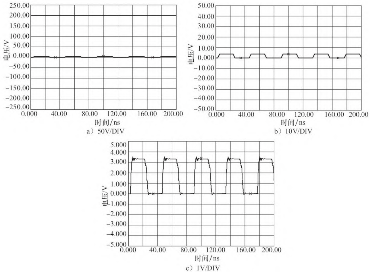
图2.31 示波器的VOLTS/DIV设置与波形
