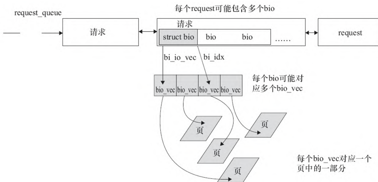
图13.3 request_queue、request、bio和bio_vec
