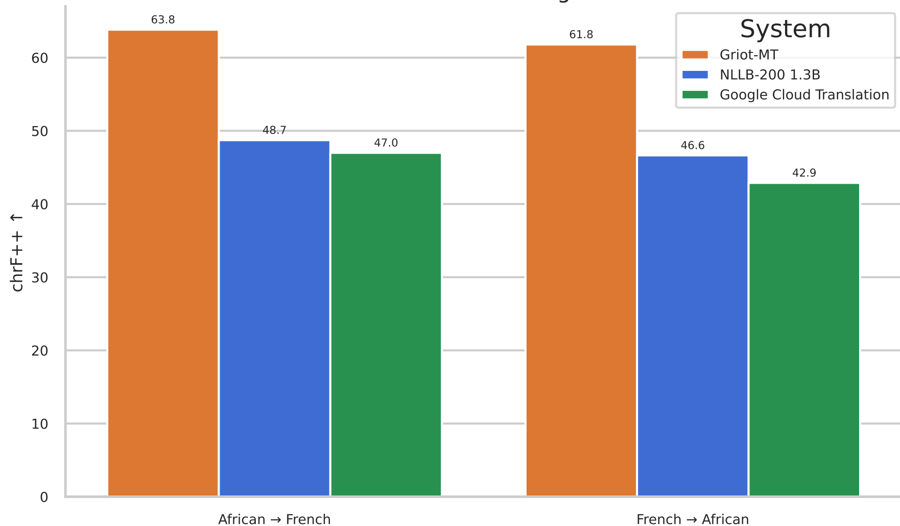
Lingala (lin) — chrF++ Griot-MT vs NLLB-200 1.3B vs Google Cloud Translation
