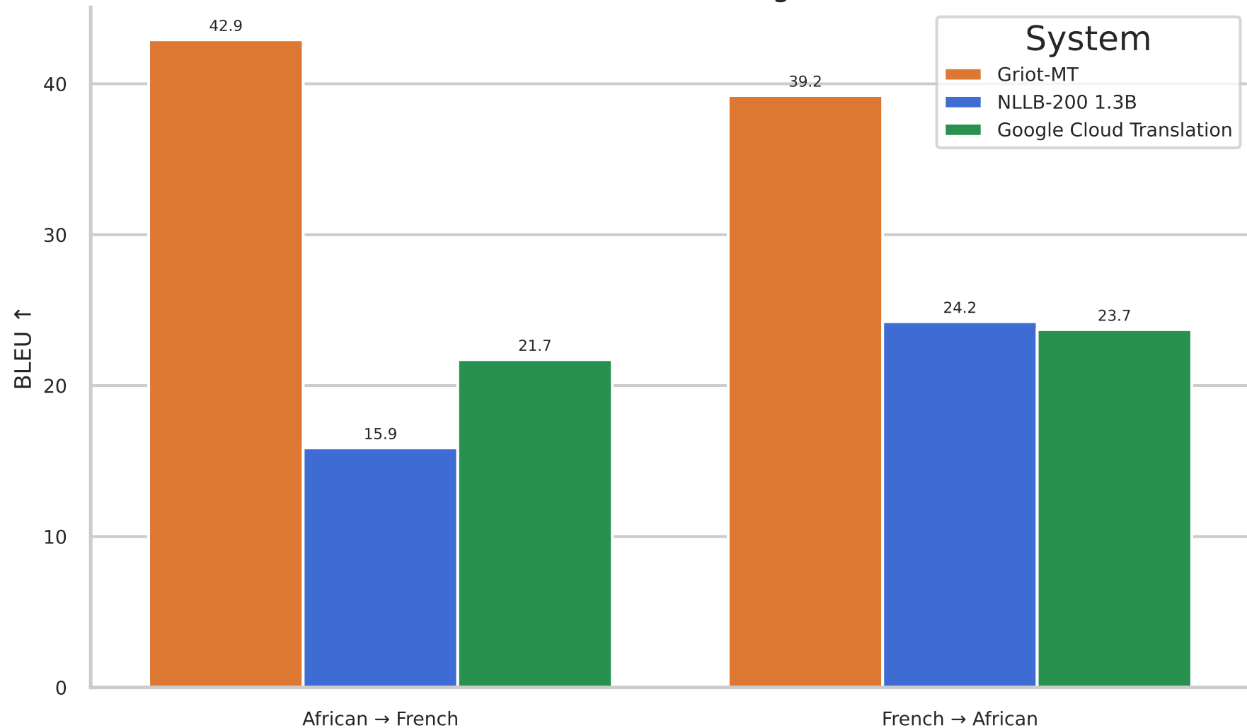
Sango (sag) — BLEU Griot-MT vs NLLB-200 1.3B vs Google Cloud Translation
