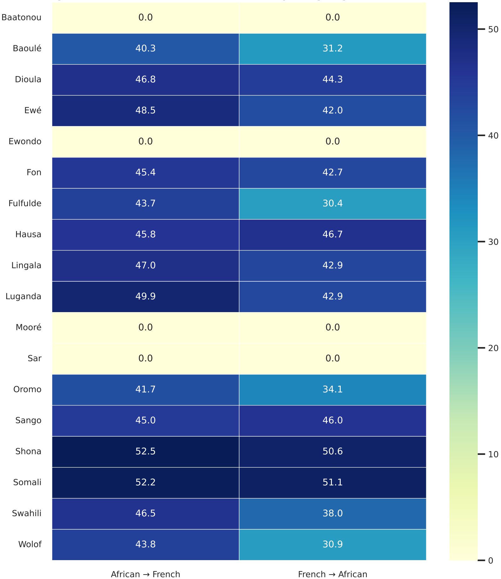
Google Cloud Translation — chrF++ by language and direction
