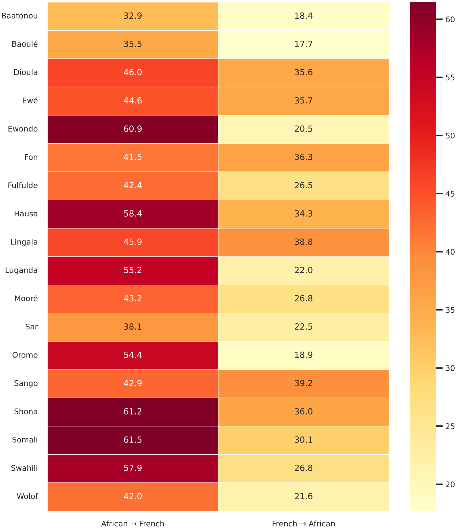
Griot-MT — BLEU by language and direction
