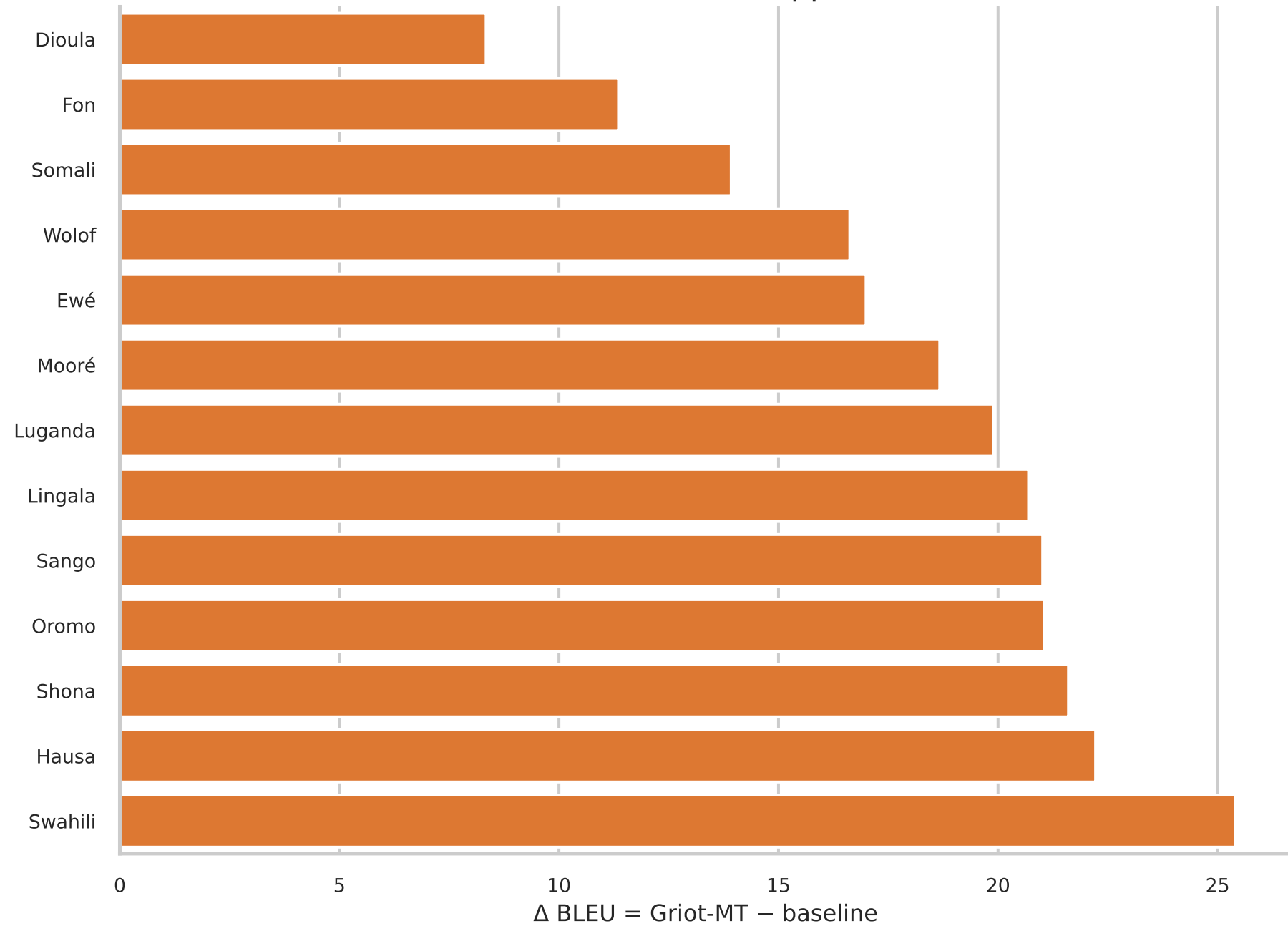
Griot-MT advantage over NLLB-200 1.3B BLEU difference on shared supported directions
