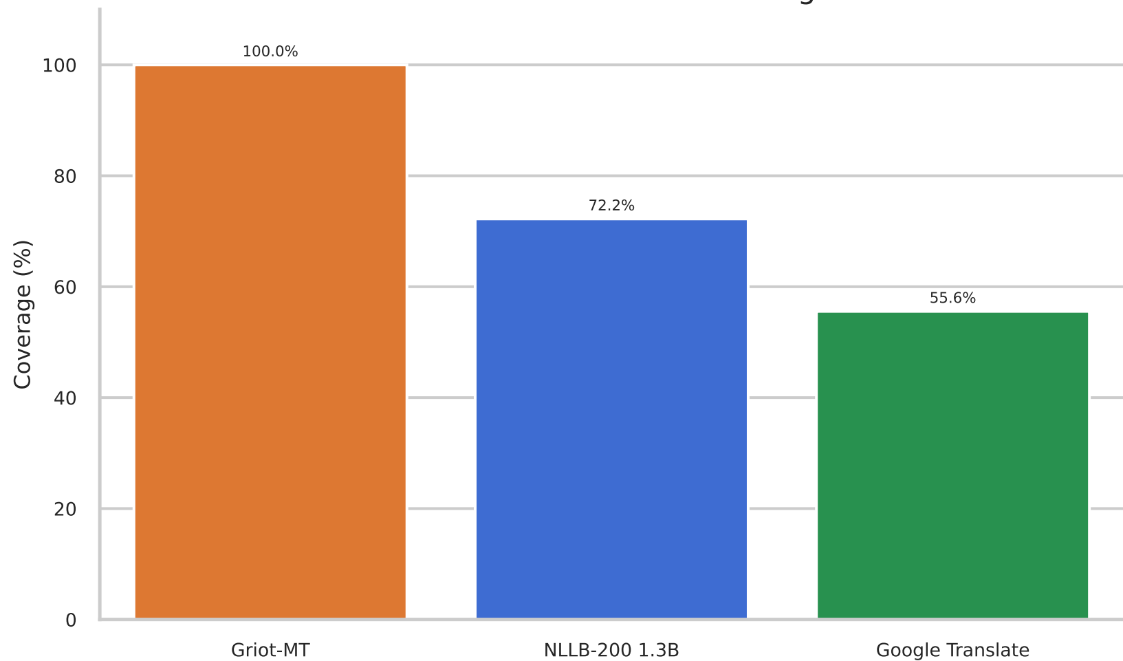
Translation-direction coverage
