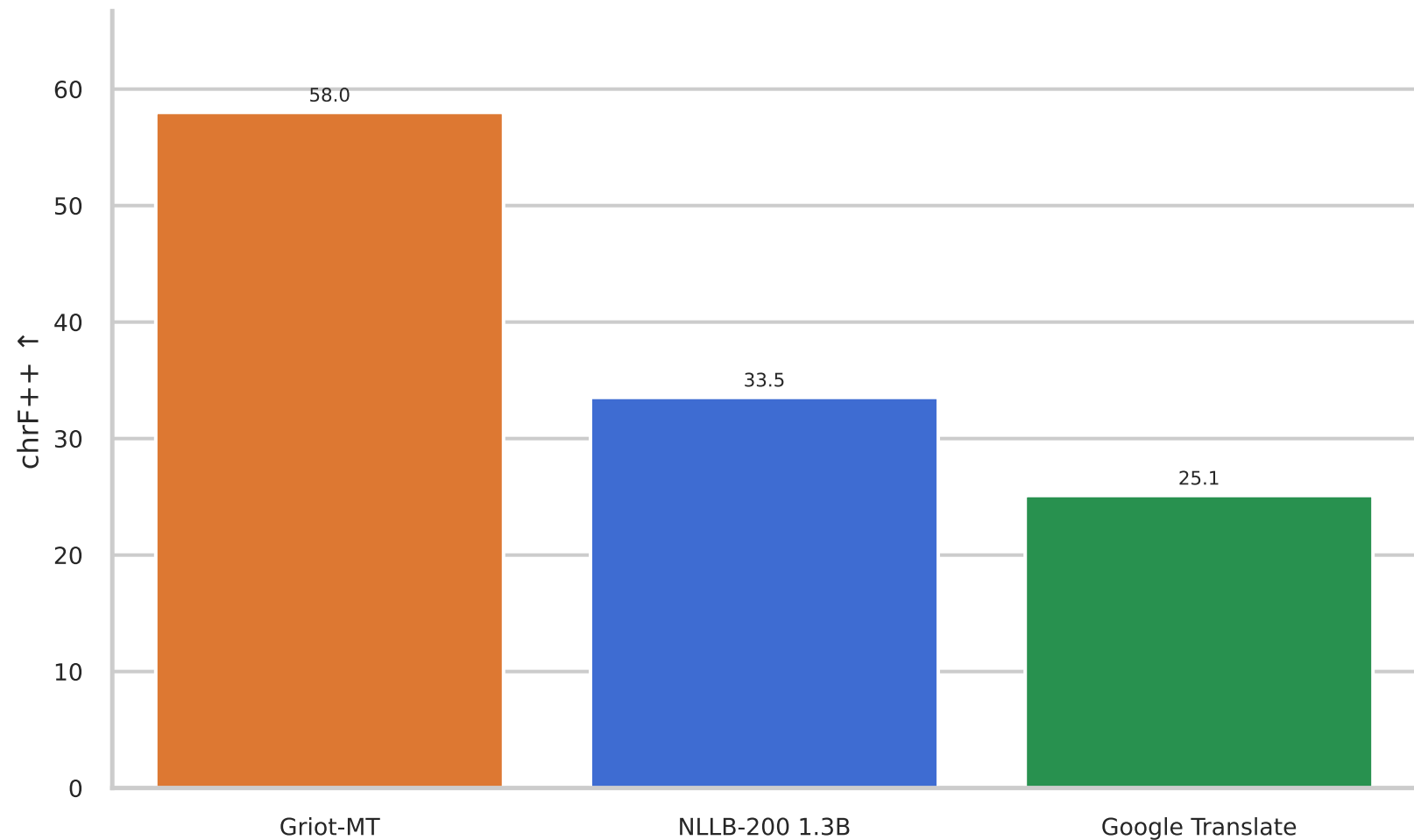
Griot-MT — Global chrF++ across 36 translation directions
