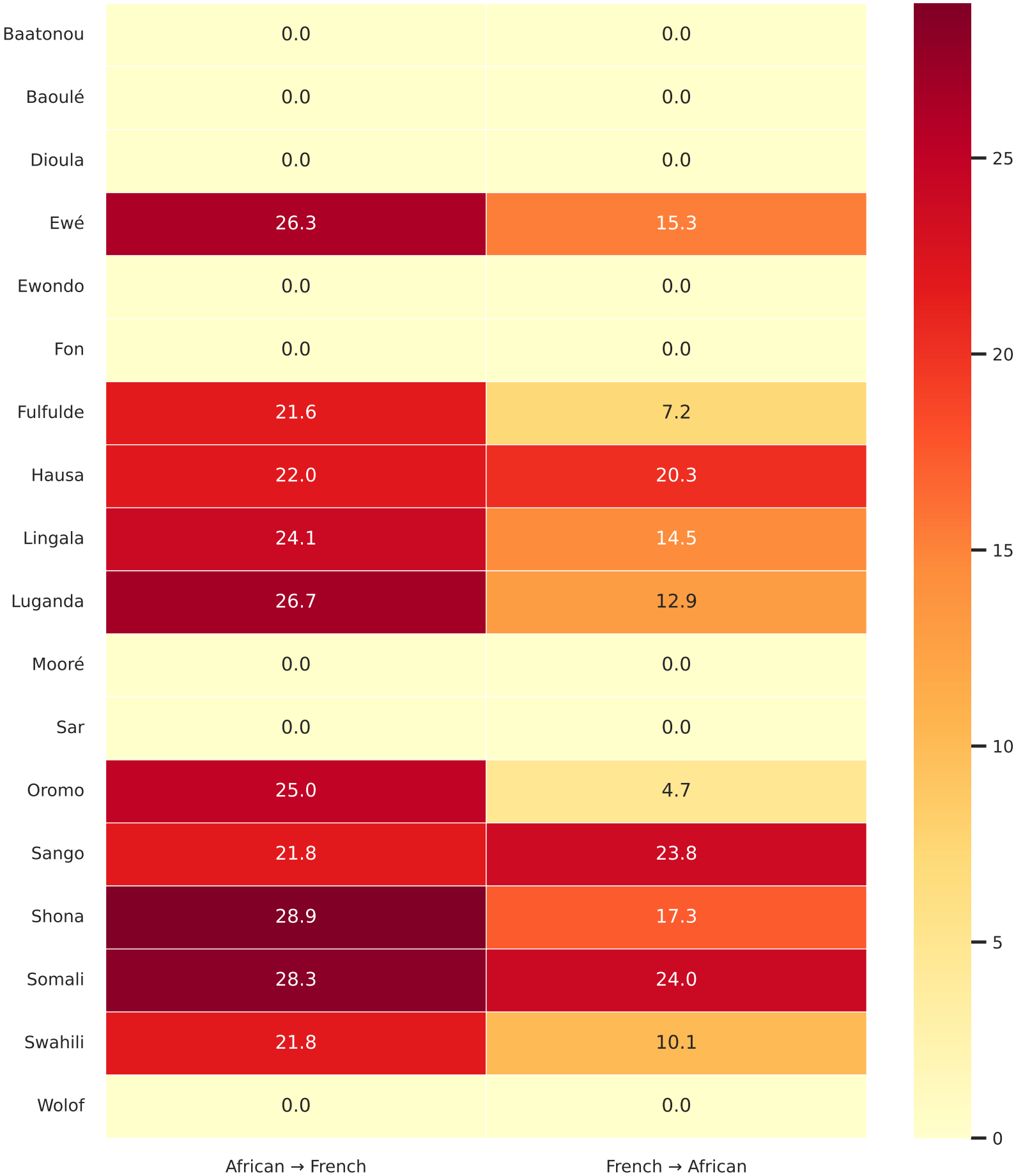
Google Translate — BLEU by language and direction
