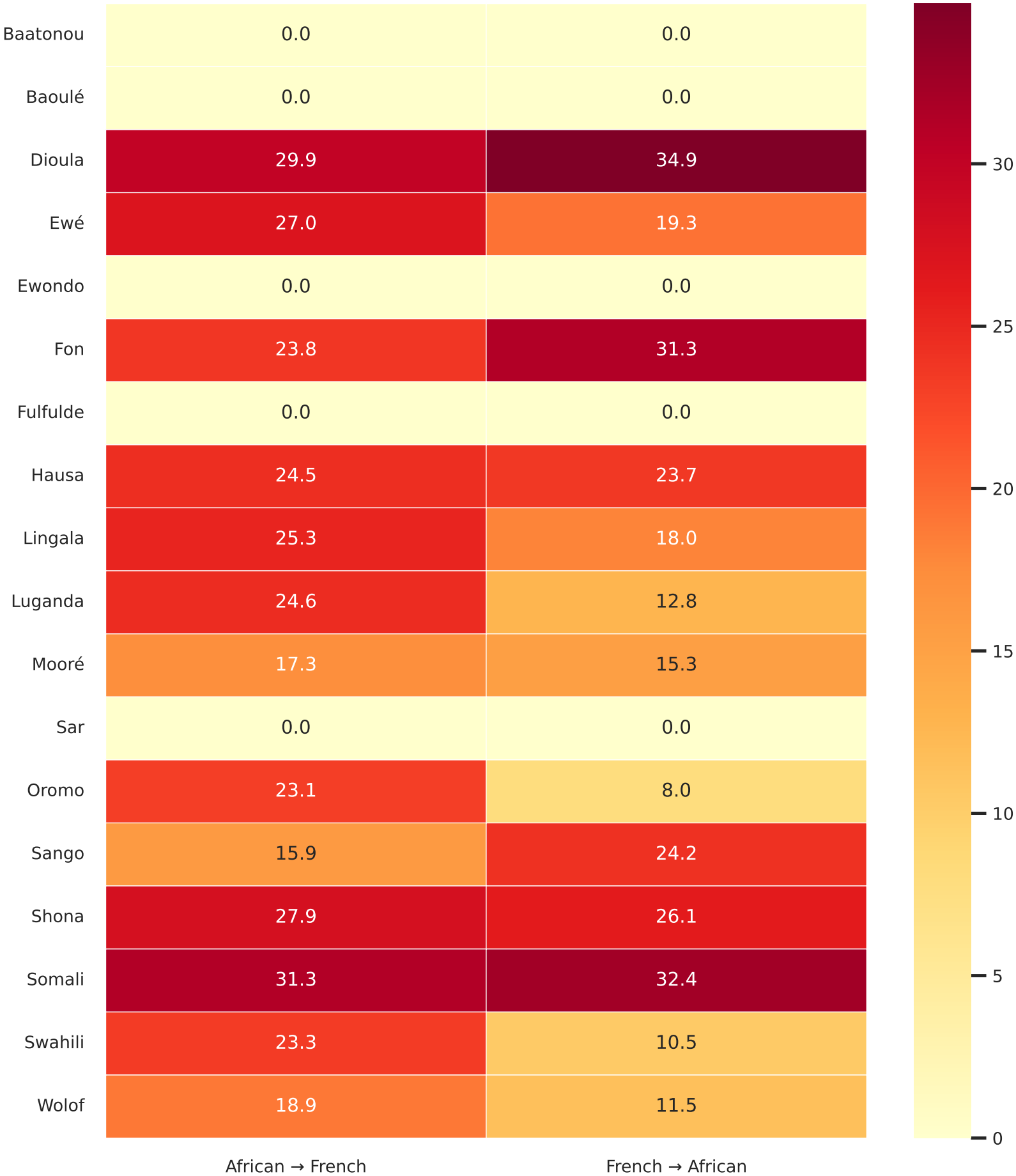
NLLB-200 1.3B — BLEU by language and direction
