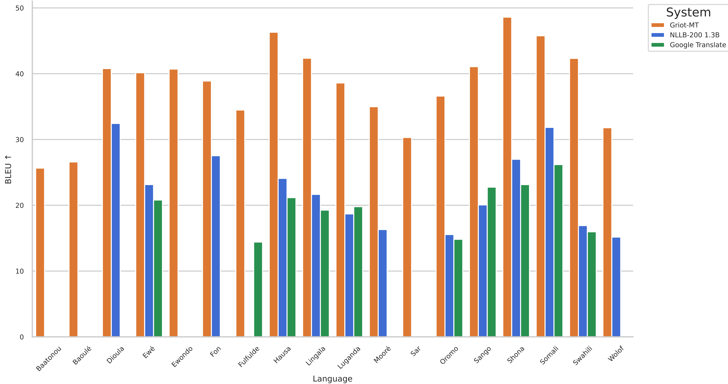
BLEU by language — average across both translation directions
