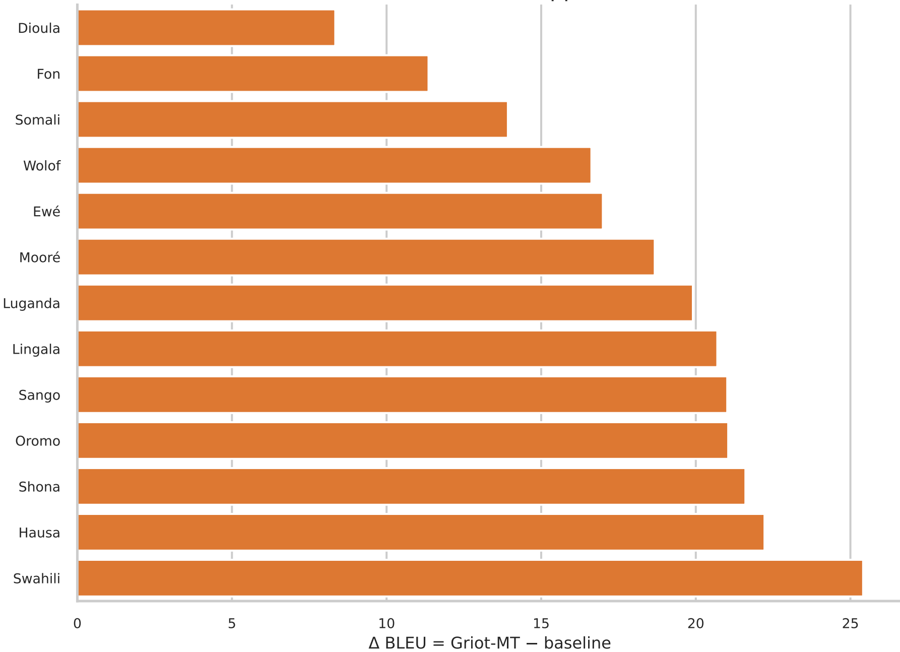
Griot-MT advantage over NLLB-200 1.3B BLEU difference on shared supported directions
