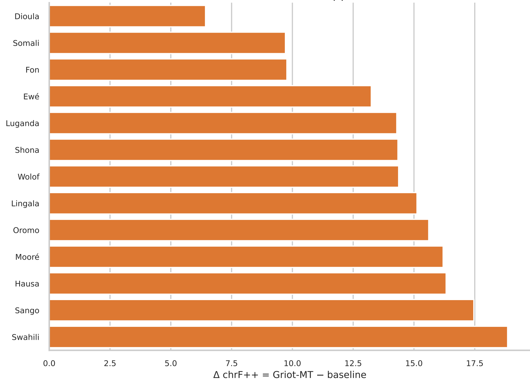
Griot-MT advantage over NLLB-200 1.3B chrF++ difference on shared supported directions
