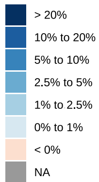
Budget gain from new taxes (in % of GNI)
