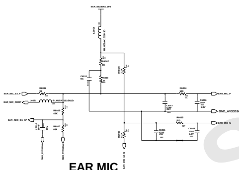
EAR MIC
