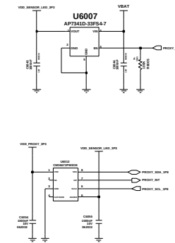
PROXIMITY SENSOR
