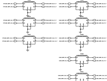
13M CAMERA FILTER
