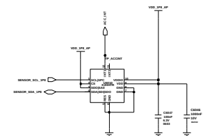
ACCELERATION SENSOR
