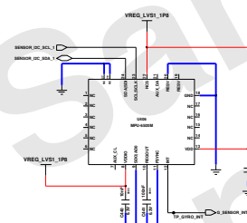
6 Axis Sensor (GYRO,ACCEL)
