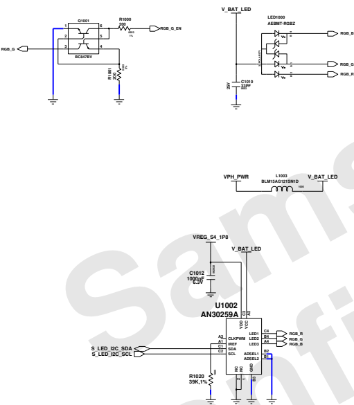
SVC LED DRIVER
