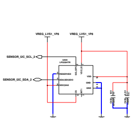
Barometer Sensor
