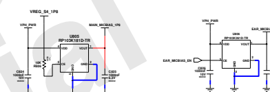
MIC Bias LDOs
