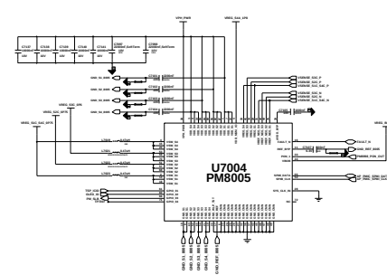
PM8005 (AP sub PMIC)
