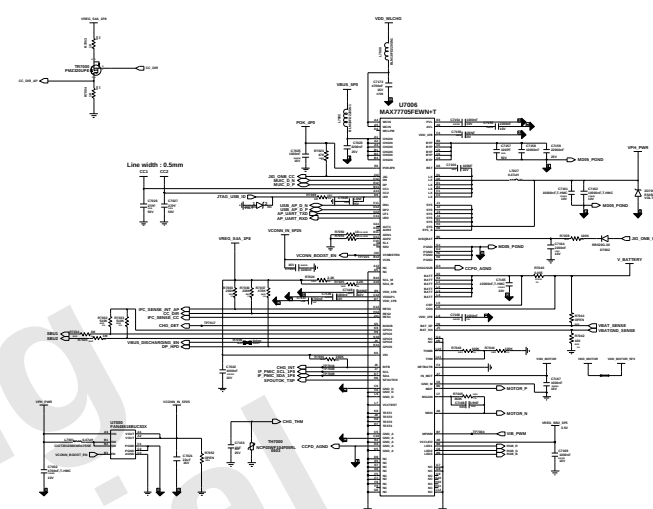
VCONN_IN_5P0 booster
