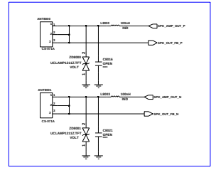
SPK CONTACT
