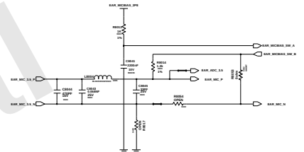
Ear MIC
