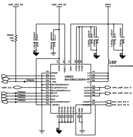
SPK AMP
