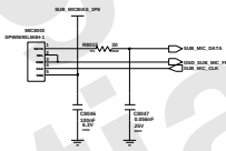
SUB MIC
