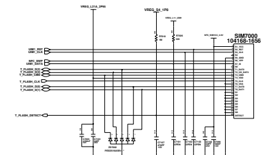
SD/SIM SOCKET
