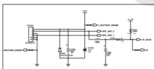
Battery Connector
