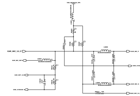
EAR_MIC
