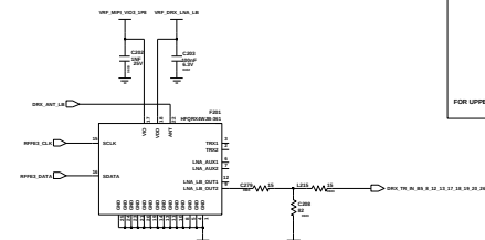
LB LFEM (B5/8/12/13/17/18/19/20/26/28)
