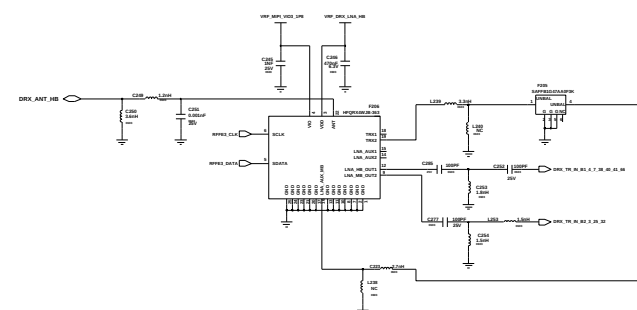
HB LFEM (B2/3/7/25/38/40/41, B1/4 4RXD)
