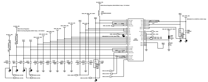
DISPLAY PMIC
