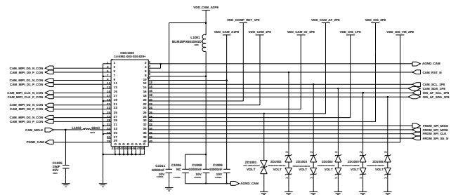
SINGLE CAMERA
