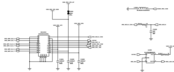
IRIS_CONNECTOR
