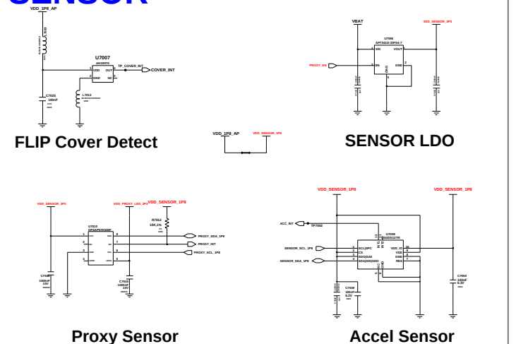
Proxy Sensor
