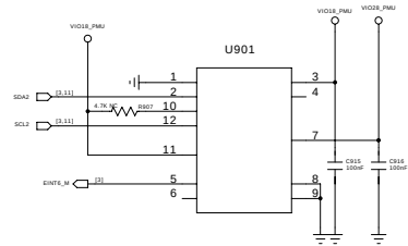
IC-ACCELEROMETER-BMA250-BOSCH
