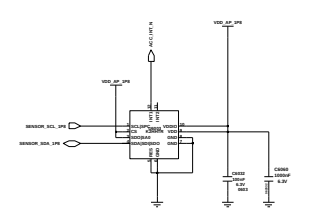
ACCELERATION SENSOR
