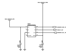
PROXIMITY SENSOR
