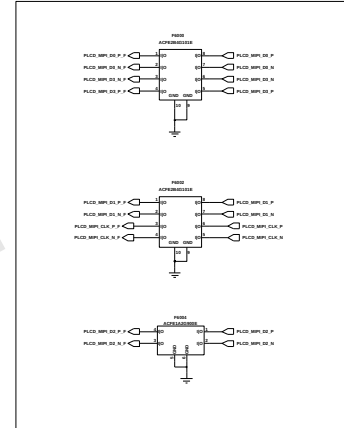
OCTA FILTER
