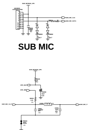
Ear MIC
