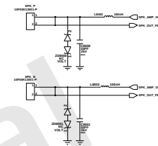
SPK CONTACT
