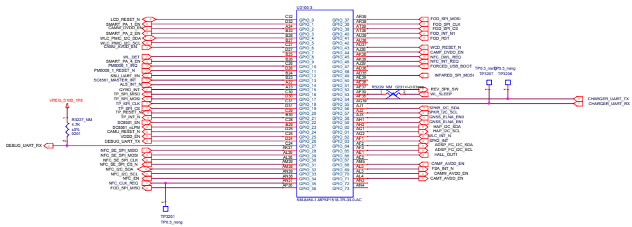
APP Processor I2C
