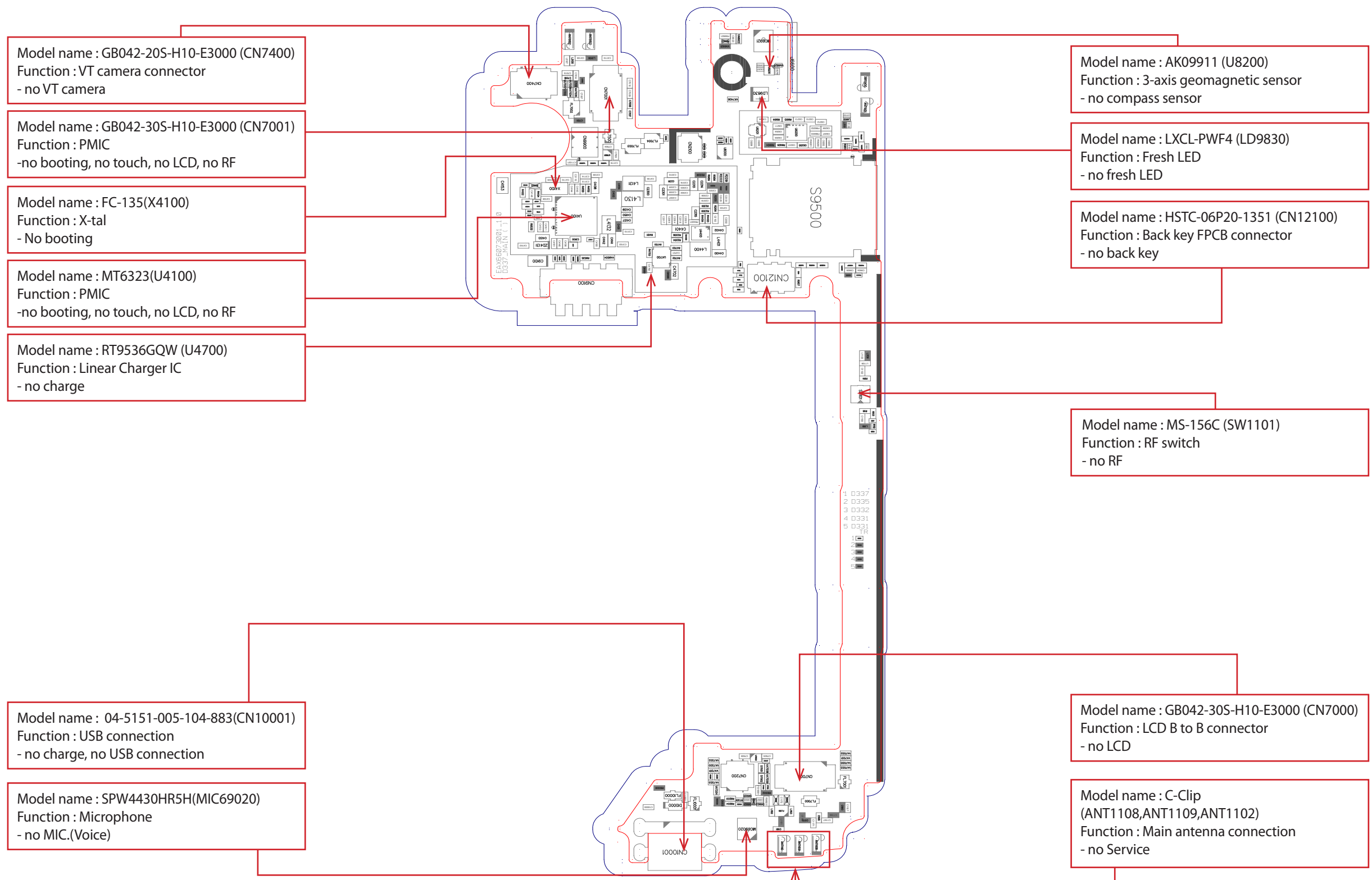
LG-D337_Main_EAX65632401_1.0_BOT-1
