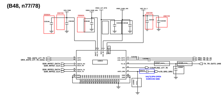
UHB (B48, n77/78)
