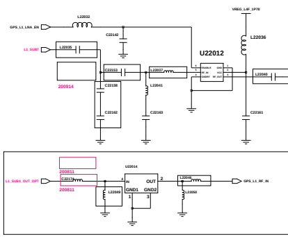
GPS_L1(for SUB4 opt)
