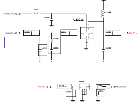
GPS_L5
