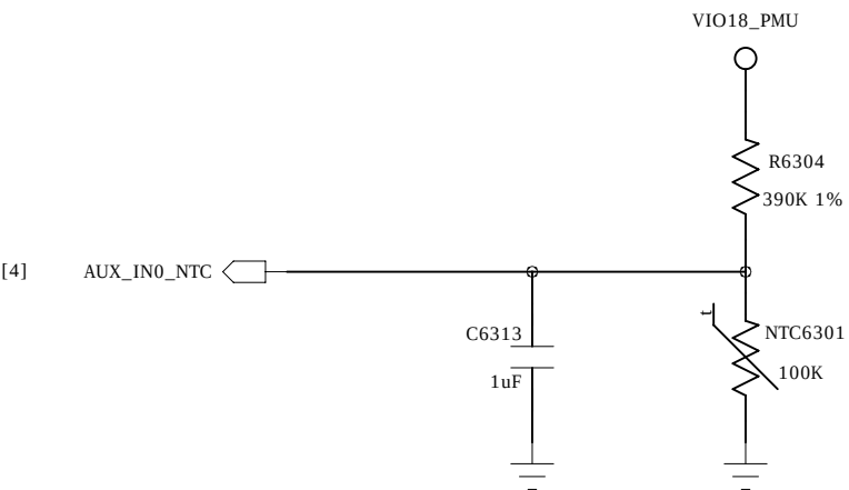
Thermister / To sense board level temperature
