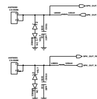
SPK CONTACT
