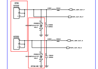
SPK CONTACT
