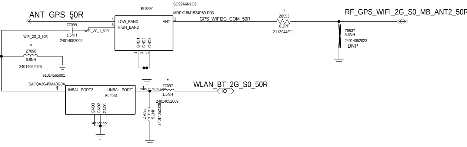
ANTENNA 2
