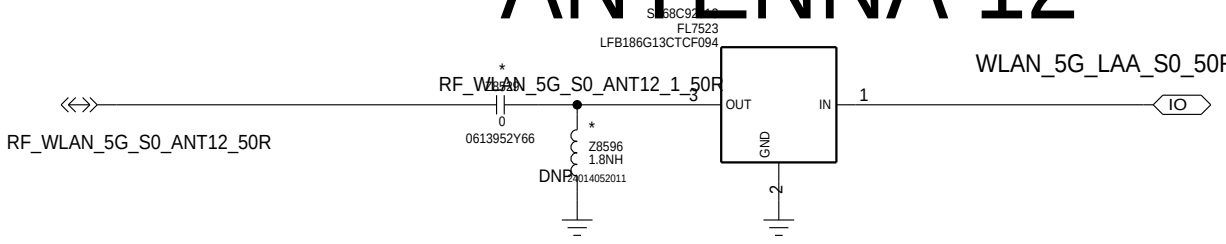
ANTENNA 12
