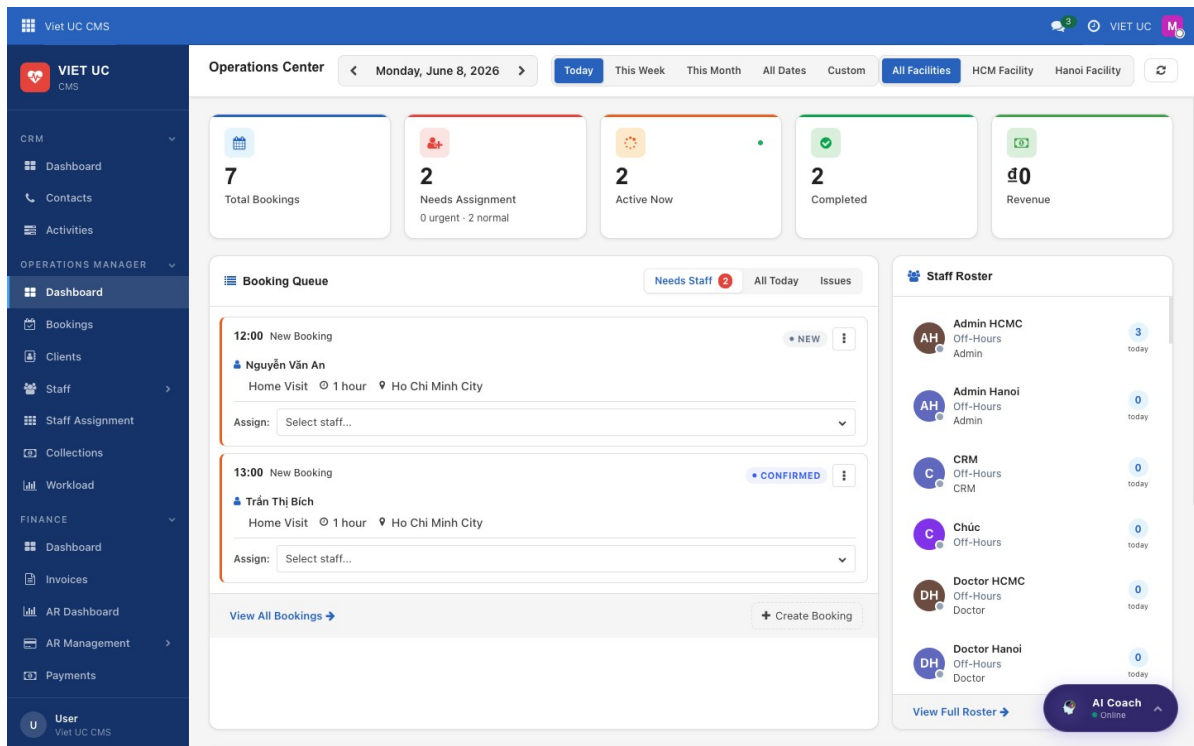
Figure: The Operations Center dashboard with KPI cards, booking queue, staff roster, and timeline
